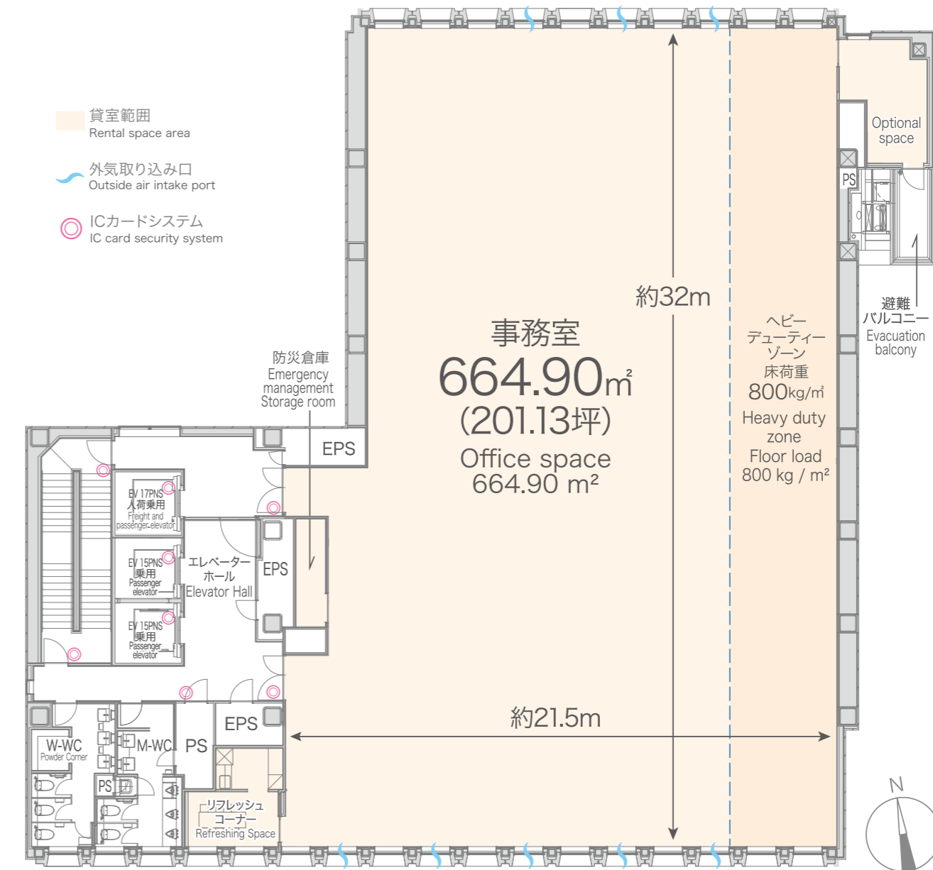
Reference floor plan view 2floor-9floor [基準階平面図(2~9階)]
